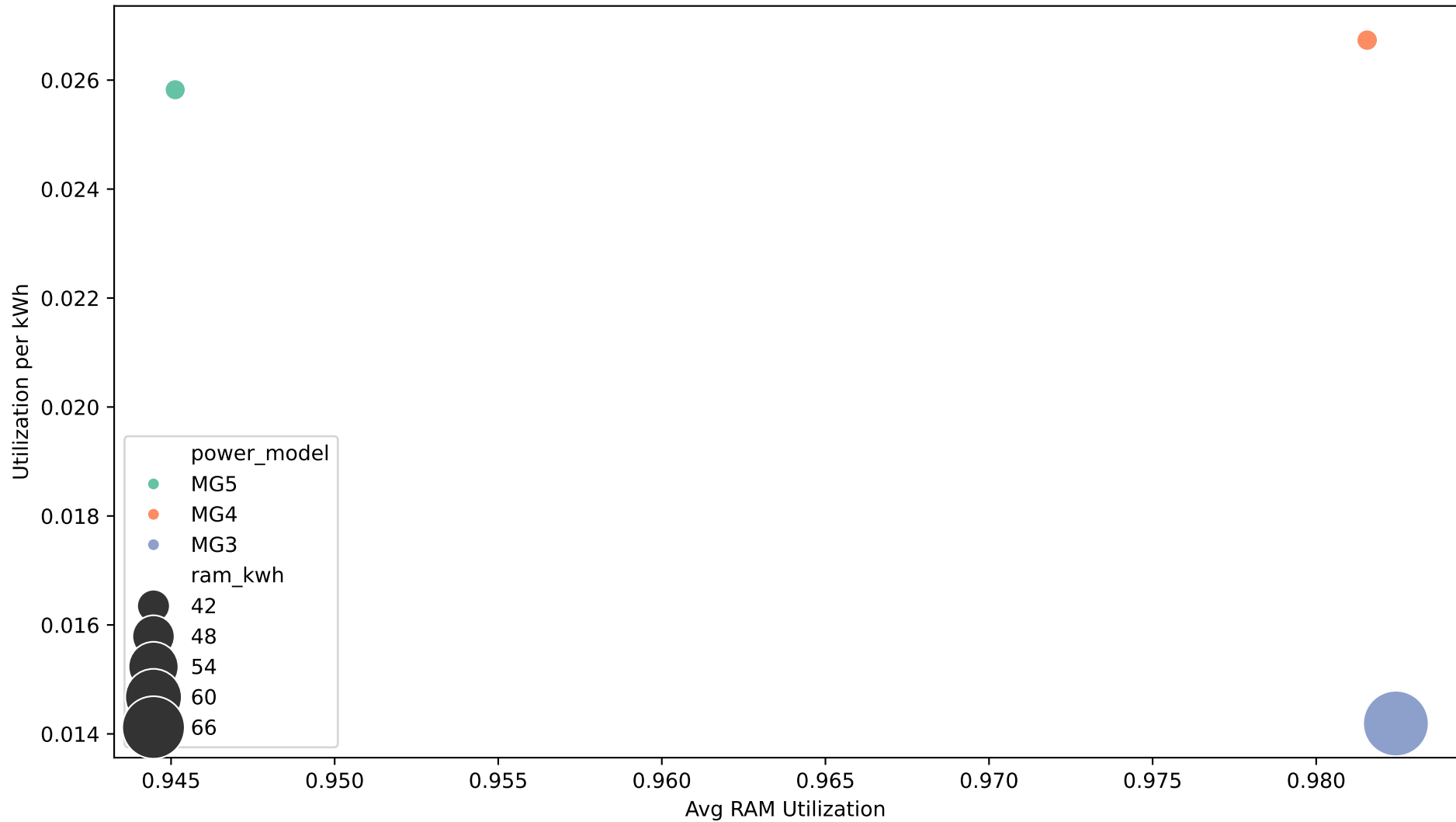
RAM Efficiency vs Utilization (Bubble = Energy Use)
